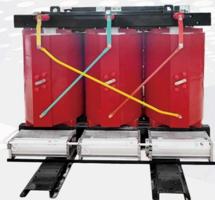
▲ Dry type transformer — Epoxy resin type
